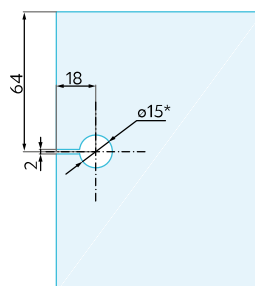
Detail C
