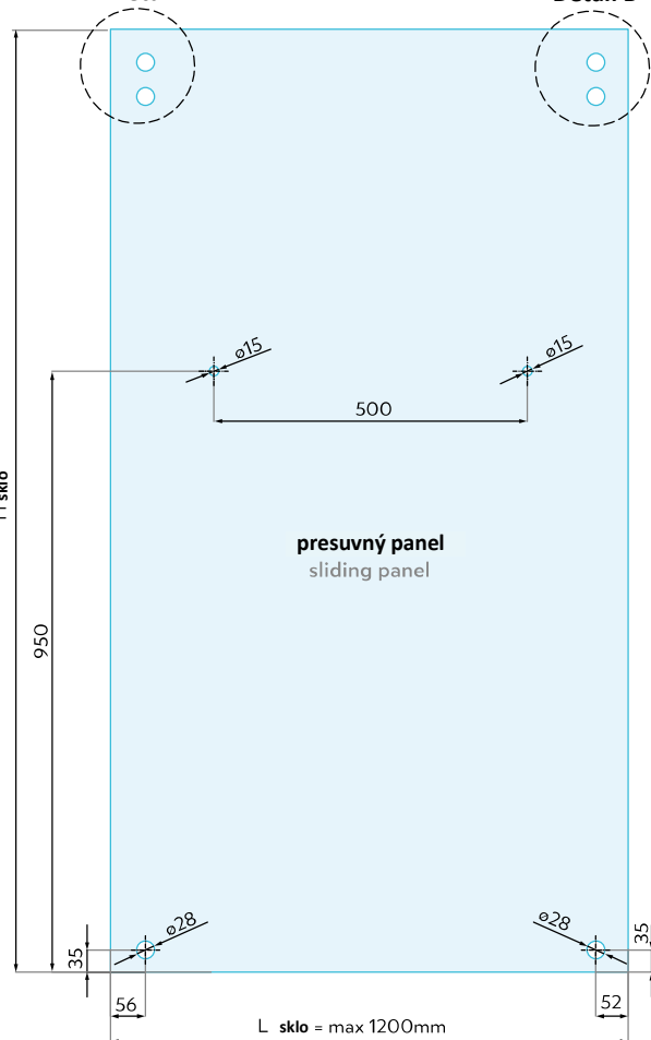
Detail A
